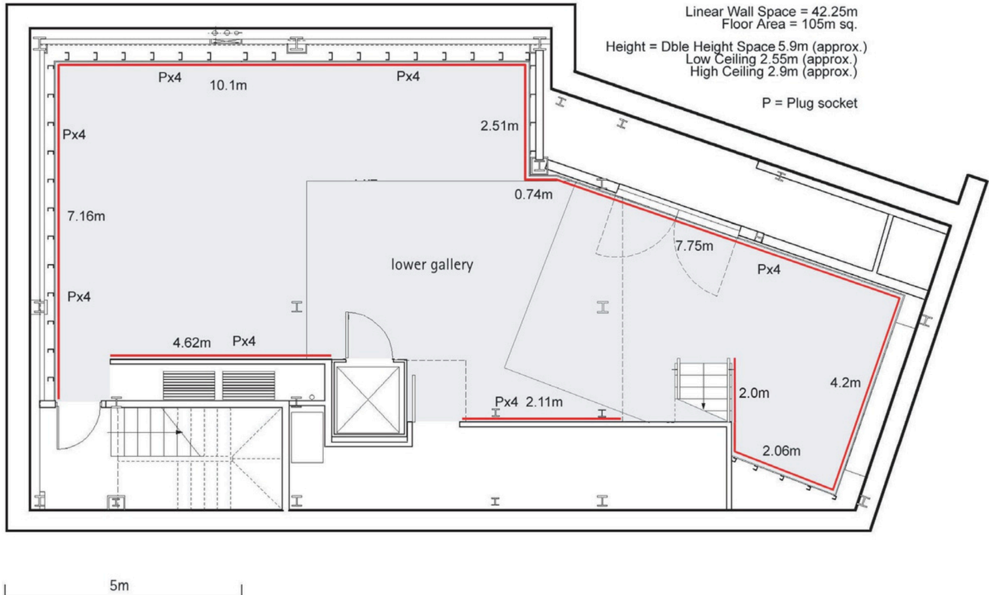
CASTLEFIELD GALLERY PLANS - LOWER GALLERY
