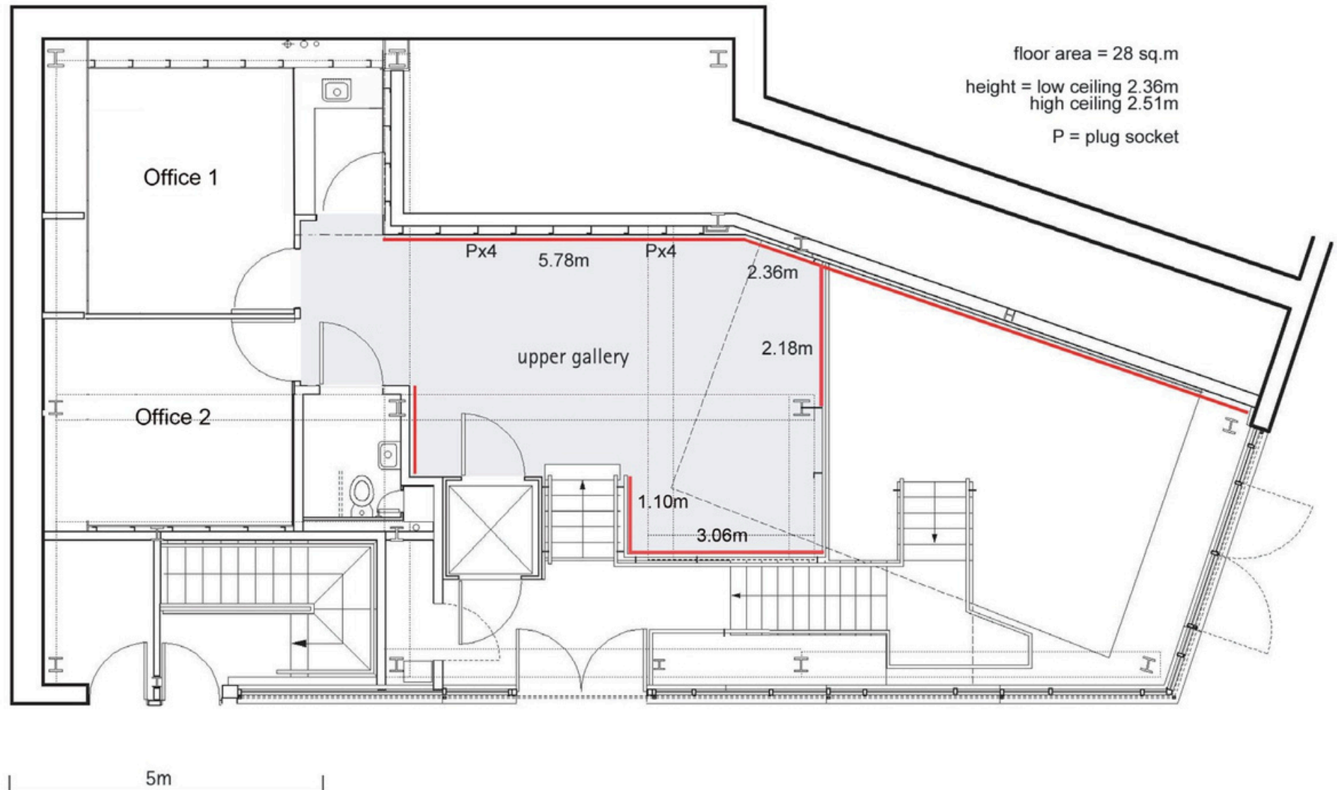
CASTLEFIELD GALLERY PLANS - UPPER GALLERY
